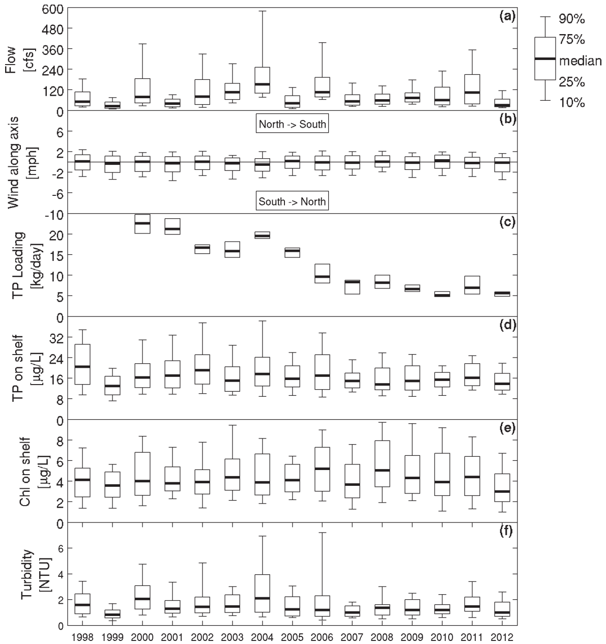
Figure 15: Comparison of study interval runoff, wind, total phosphorus loading, total phosphorus concentration, Chlorophyll-a concentration and turbidity. Legend marks percentile range of data. (a) Fall Creek flow, (b) wind speed, (c) summed loads of total phosphorus (TP) from the IAWWTF, CHWWTP and the LSC facility, (d) total phosphorus concentration on the south shelf, (e) Chlorophyll-a concentration on the south shelf, and (f) turbidity on the south shelf. Data plotted are from the May - October interval. Shelf data includes measurements from sites 1, 3, 4, 5 and 7.
