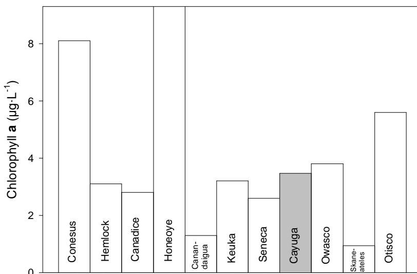
Figure 10. Comparison of average chlorophyll a concentrations for the spring-early fall interval for the eleven Finger Lakes, based on samples (n=15 to 16) collected over the 1996 through 1999 interval (data from Callinan et al. 2000).
