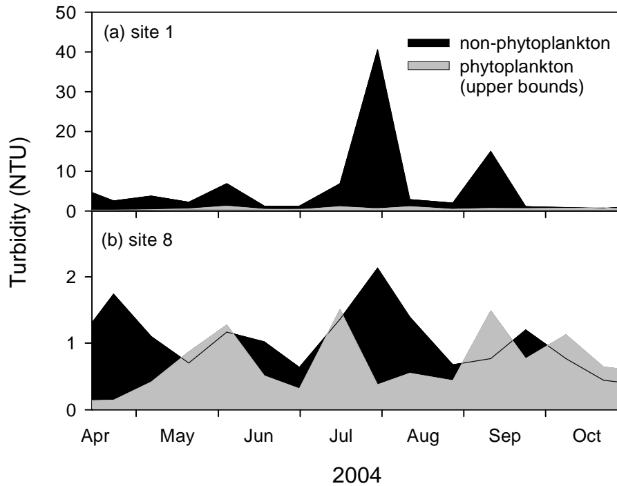
Figure 9. Time-series of T_n and contributions from components (phytoplankton and non-phytoplankton) for the April – October interval of 2004: (a) site 1, and (b) site 8.
