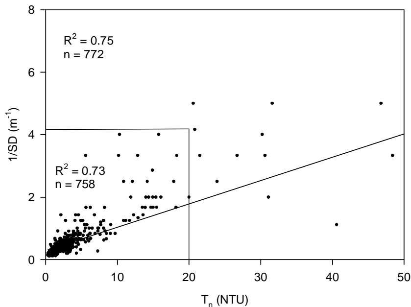
Figure 4. Relationship between Secchi disc transparency (SD) and turbidity in the southern end of Cayuga Lake based on paired measurements made during the 1998 – 2004 study interval.
