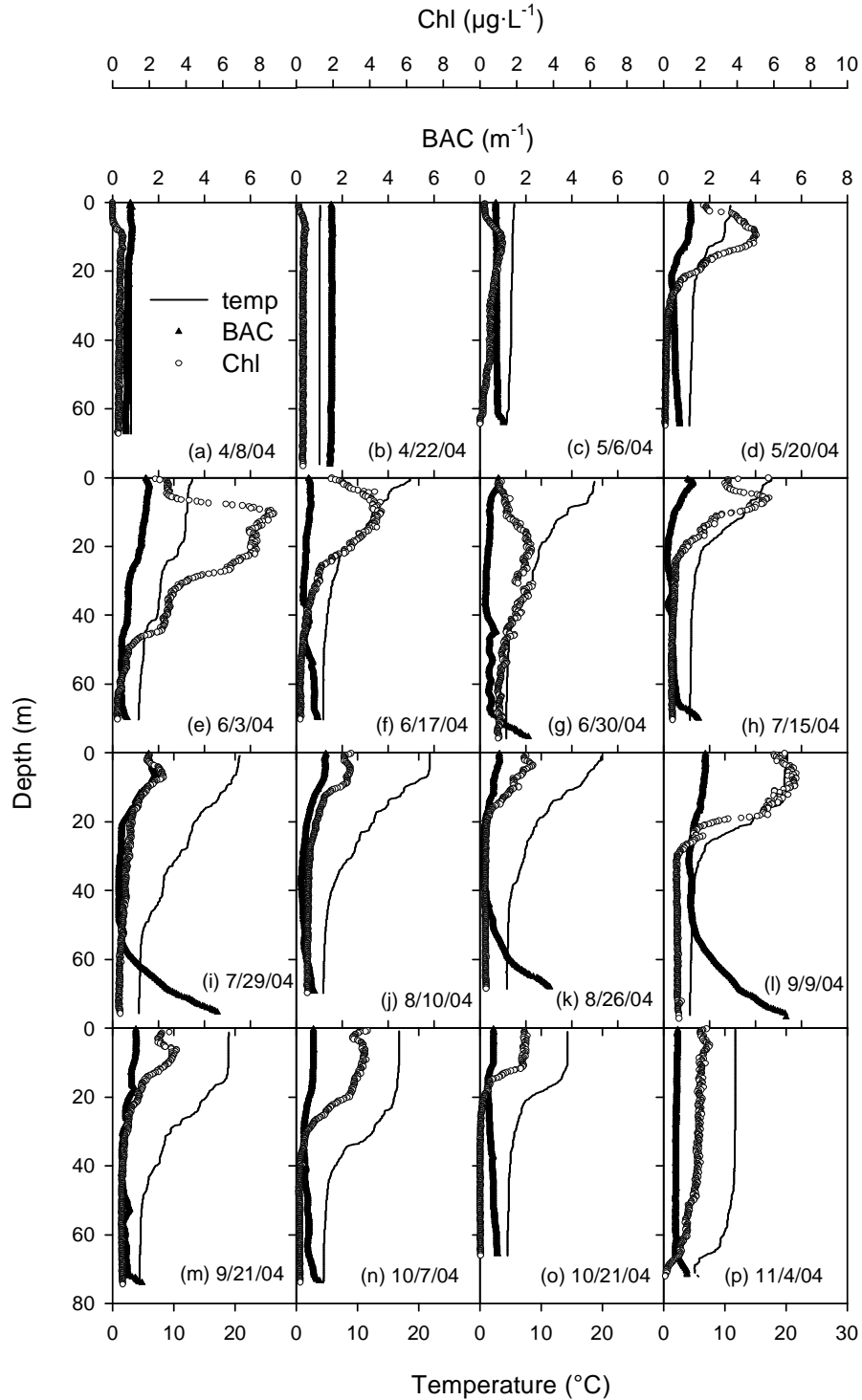
Figure 3. Vertical profiles of temperature, chlorophyll fluorescence, and beam attenuation coefficient (BAC) for LSC site in 2004: (a) April 8, (b) April 22, (c) May 6, (d) May 20, (e) June 3, (f) June 17, (g) June 30, (h) July 15, (i) July 29, (j) August 10, (k) August 26, (l) September 9, (m) September 21, (n) October 7, (o) October 21, and (p) November 4.
