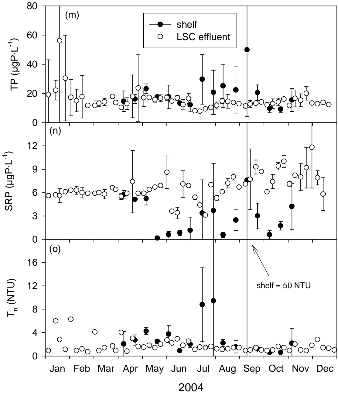
Figure 2m-o. Time series of parameter values for the south shelf and the LSC effluent for 2004: (m) TP, (n) SRP, and (o) T_n . Results for the “shelf” are averages; the error bars represent spatial variation with dimensions of \pm 1 standard deviation. Error bars for the LSC effluent represent 95% confidence intervals determined from analyses of field triplicates.
