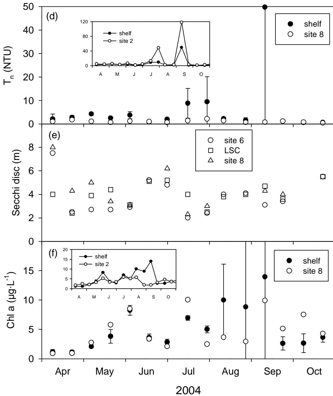
Figure 2d-f. Time series of parameter values for Cayuga Lake for 2004: (d) T_n , (e) Secchi disc, and (f) Chl a. Insets present results for site 2. Results for the “shelf” are averages; the error bars represent spatial variation with dimensions of \pm 1 standard deviation.
