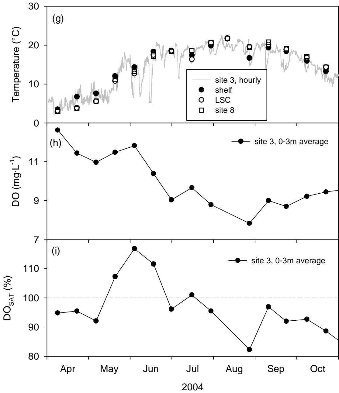
Figure 2g-i. Time series of parameter values for Cayuga Lake for 2004: (g) temperature, (h) DO, and (i) DO SAT .
