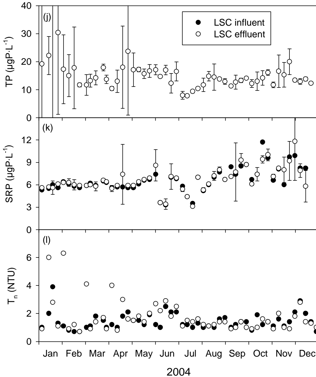
Figure 2j-1. Time series of parameter values for the LSC influent and effluent for 2004: (j) TP, (k) SRP, and (l) T_n . Error bars represent 95% confidence intervals determined from analyses of field triplicates.
