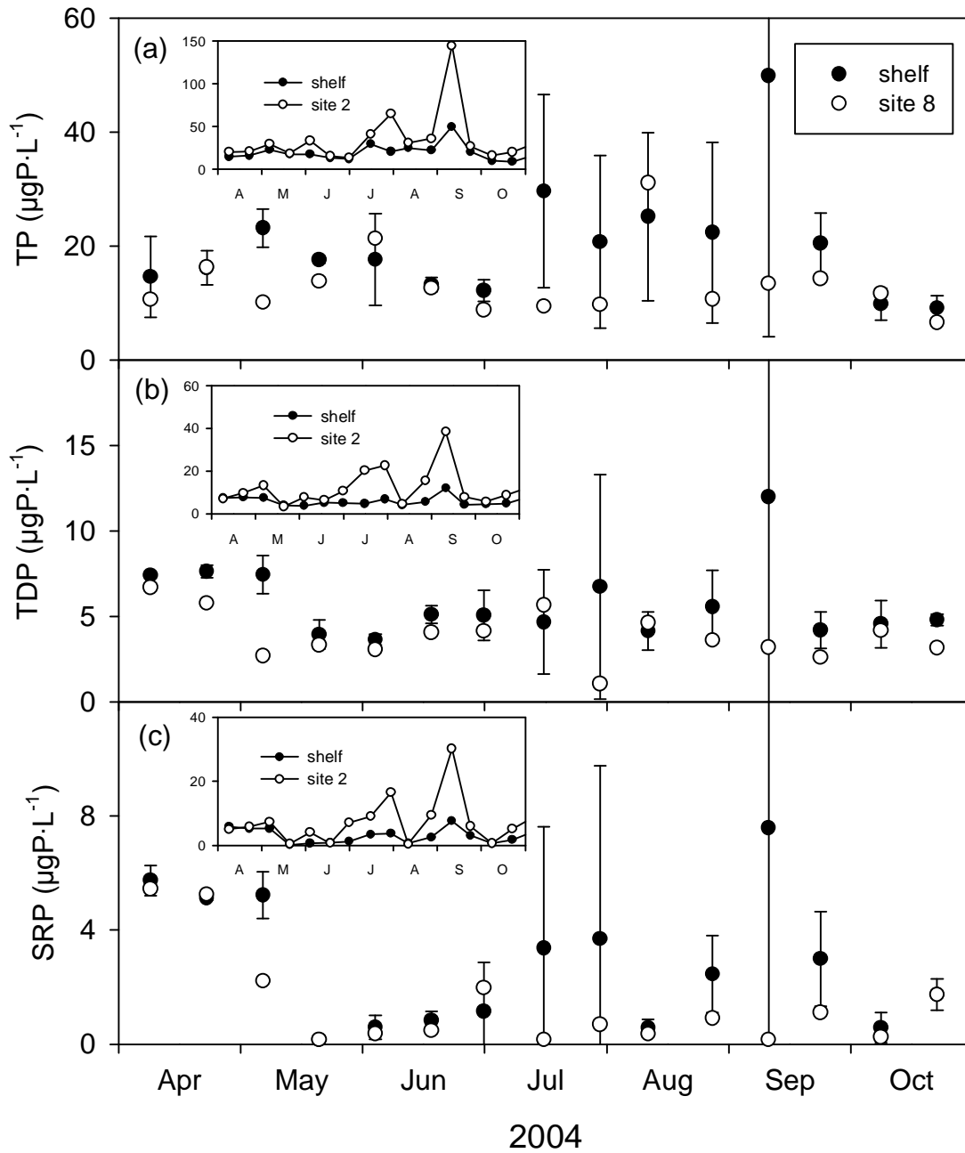
Figure 2a-c. Time series of parameter values for Cayuga Lake for 2004: (a) TP, (b) TDP, and (c) SRP. Insets present results for site 2. Results for the “shelf” are averages; the error bars represent spatial variation with dimensions of \pm 1 standard deviation.
