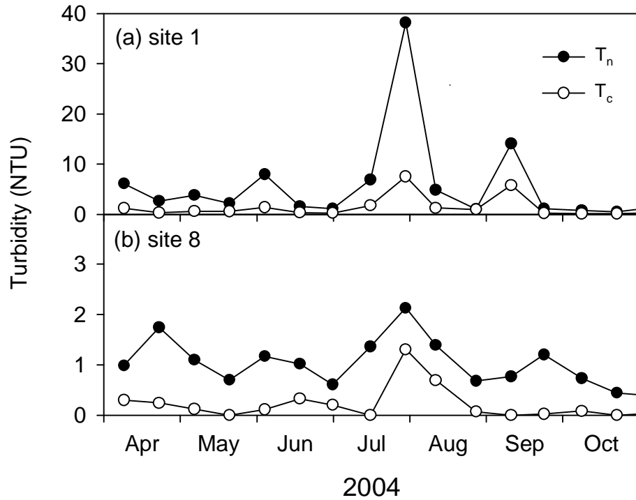
Figure 7. Distributions of total turbidity ( T_n ) and calcium carbonate turbidity ( T_c ) in the upper waters of Cayuga Lake in 2004: (a) site 1, (b) site 8.
