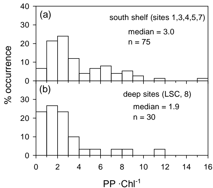
Figure 8. Distributions of the particulate P (PP) to chlorophyll a ratio values in Cayuga Lake in 2004: (a) south shelf sites, and (b) deep water sites.
